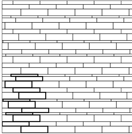
TTS60-1 11% /m 2 5 x 60 cm / 2 x 24 inch 31% /m 2 10 x 60 cm / 4 x 24 inch 58% /m 2 15 x 60 cm / 6 x 24 inch
