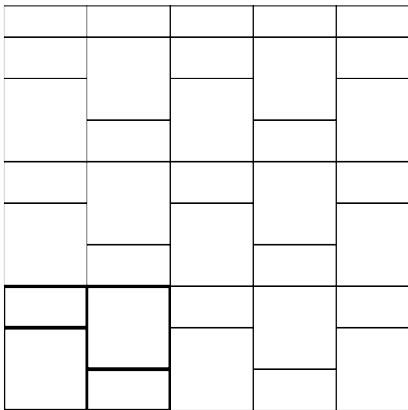
TTS60-6 33% /m 2 30 x 60 cm / 12 x 24 inch 67% /m 2 60 x 60 cm / 24 x 24 inch
