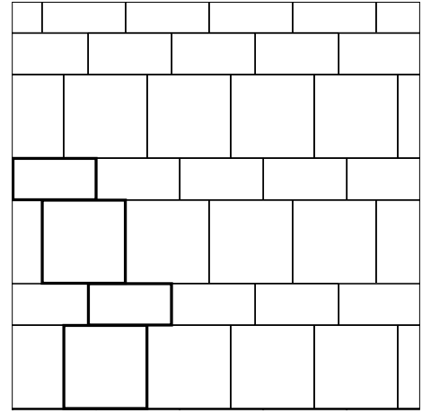
TTS60-7 33% /m 2 30 x 60 cm / 12 x 24 inch 67% /m 2 60 x 60 cm / 24 x 24 inch
