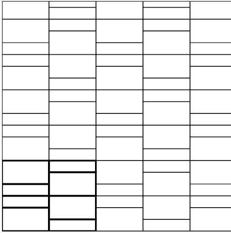
TTS60-4 33% /m 2 15 x 60 cm / 6 x 24 inch 67% /m 2 30 x 60 cm / 12 x 24 inch
